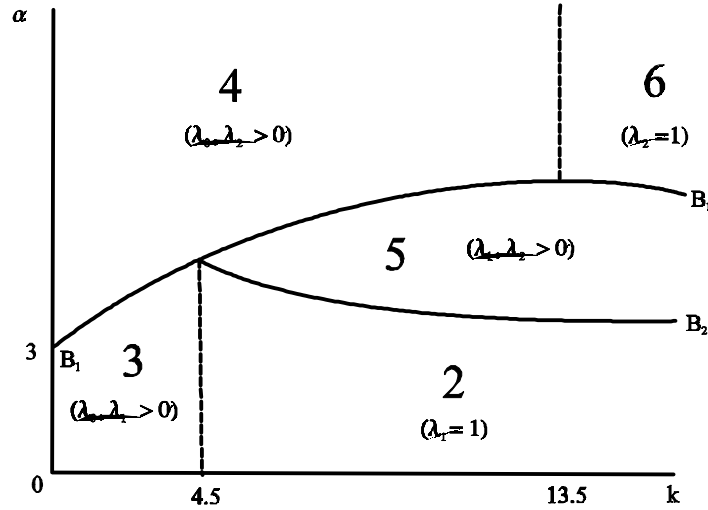
Figure 3: Phase Diagram: Capitalists
