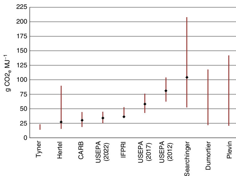
Figure 2 Ranges of results from models of ILUC emissions induced by expansion of corn ethanol production. Point estimates are indicated by the diamond where applicable. USEPA estimated ILUC emissions that would occur to meet the US Renewable Fuel Standard in each of three years: 2012, 2017, and 2022 (Tyner et al. , 2010; Hertel et al. , 2010; CARB, 2009; USEPA, 2010; IFPRI = Al-Riffai et al. , 2010; Searchinger et al. , 2008; Dumortier et al. , 2009, and Plevin et al. , 2010).
