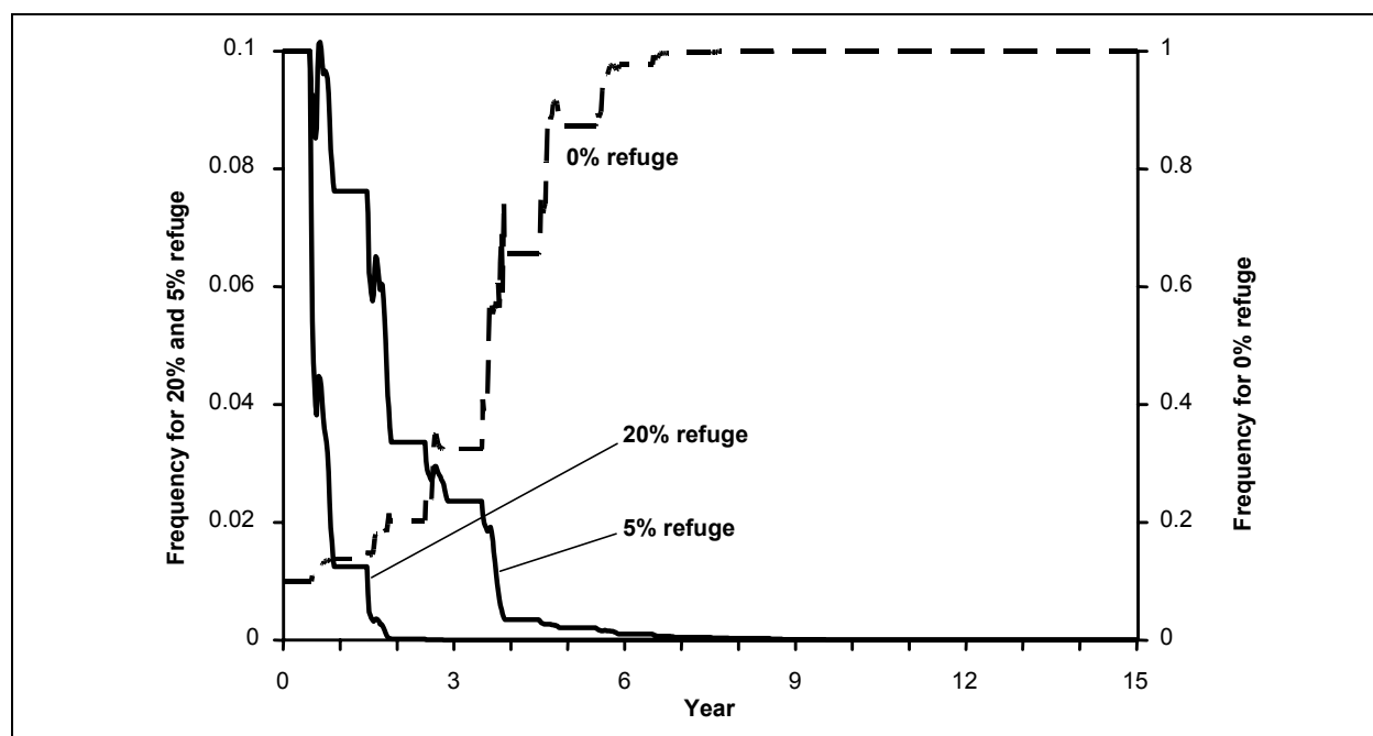
Figure 2. Simulation of Bt resistance development in bollworm population.
